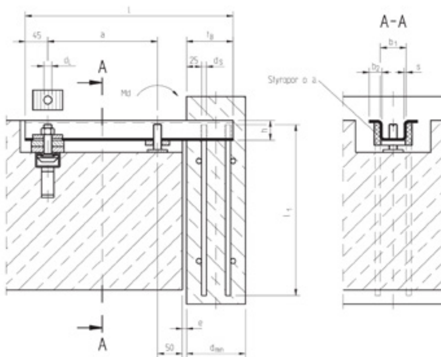
Parapet anchor, with adjustment screw, roof unit, Part no. 04BA205- Md -L
